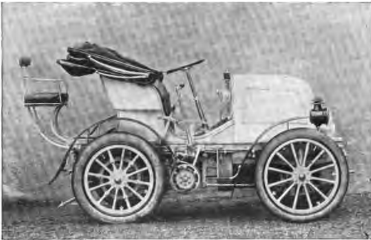
FIG. 871.—Two-seated Pleasure Carriage for general use; built by the Cannstadt-Daimler Co.
